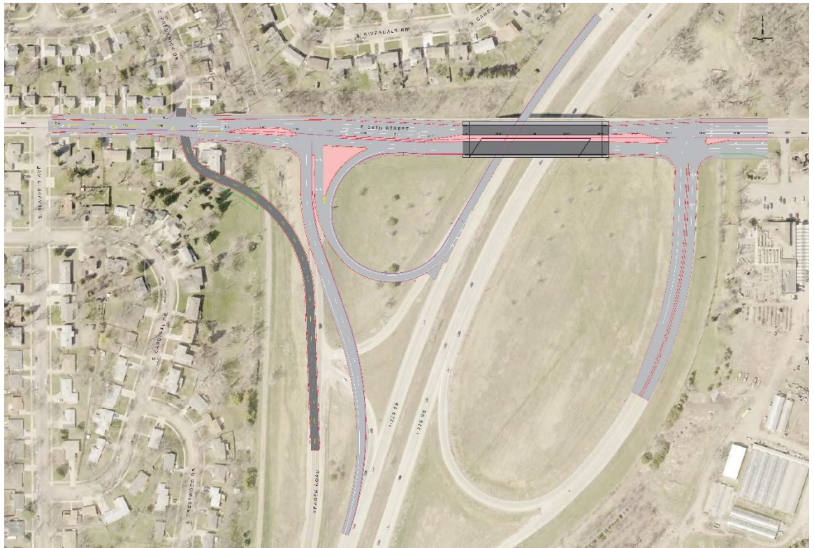
Figure 10 – Proposed I-229 at 26 th Street Interchange (2020)
