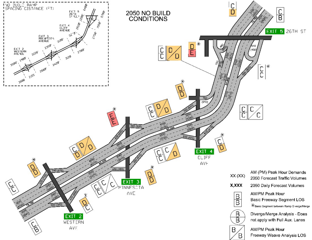
Figure 26 – 2050 No Build Freeway Configuration and LOS
